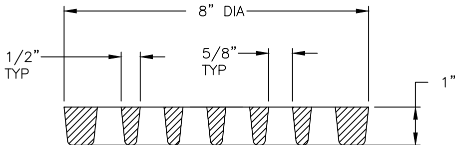
GRATE SECTION
